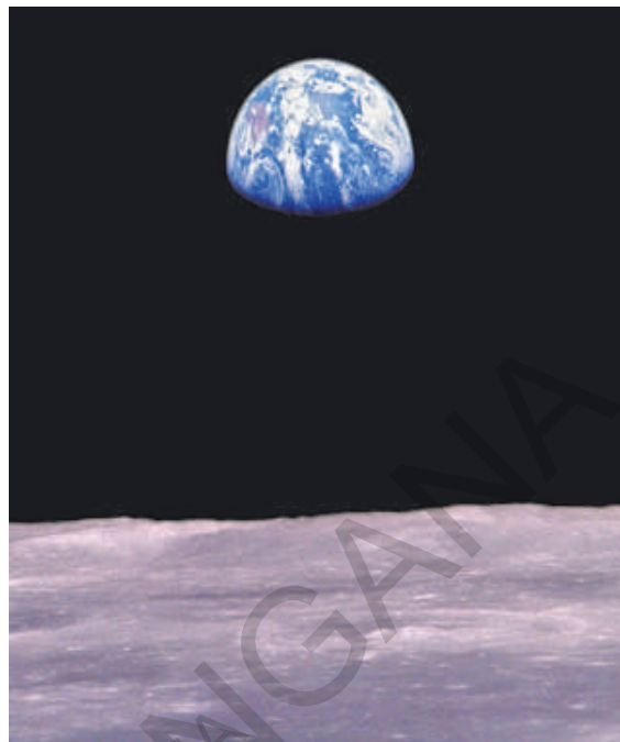
Fig 3.4: A view of the earth from the Moon
